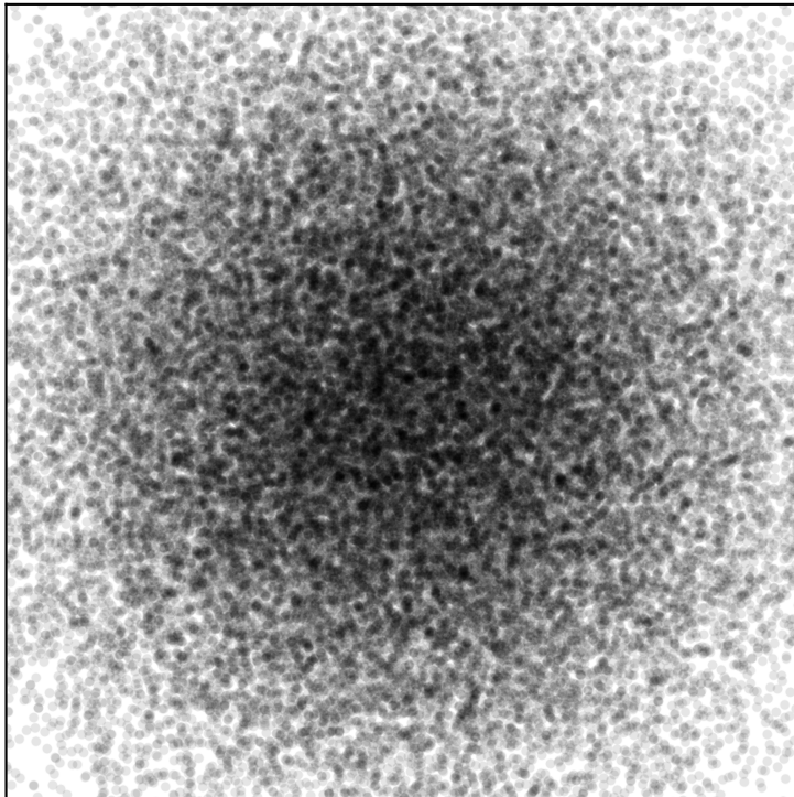
Scatter/Image plot (n=50,000)
