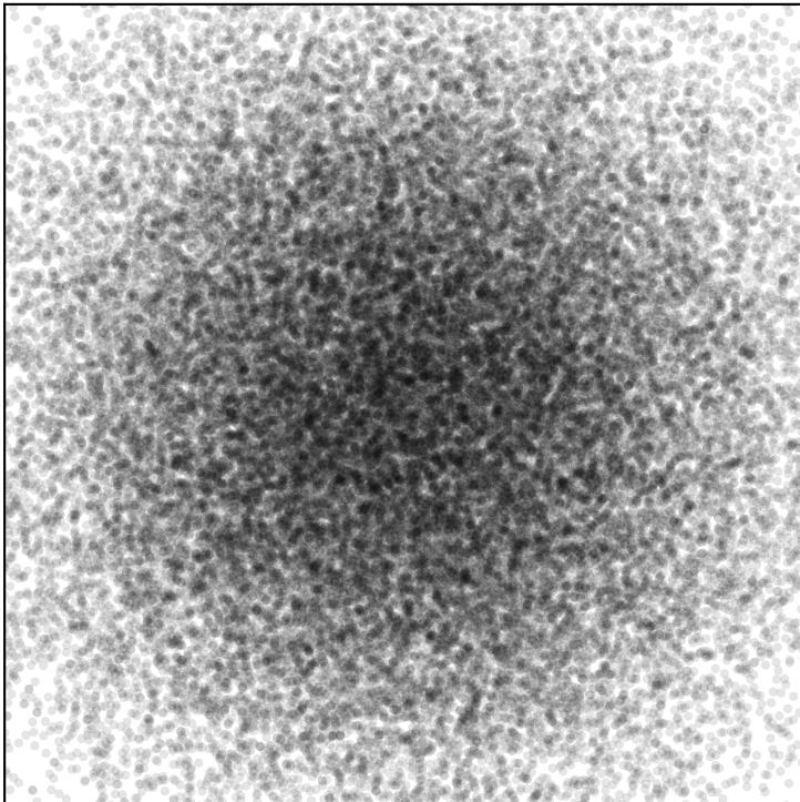
Scatter plot (n=50,000)
